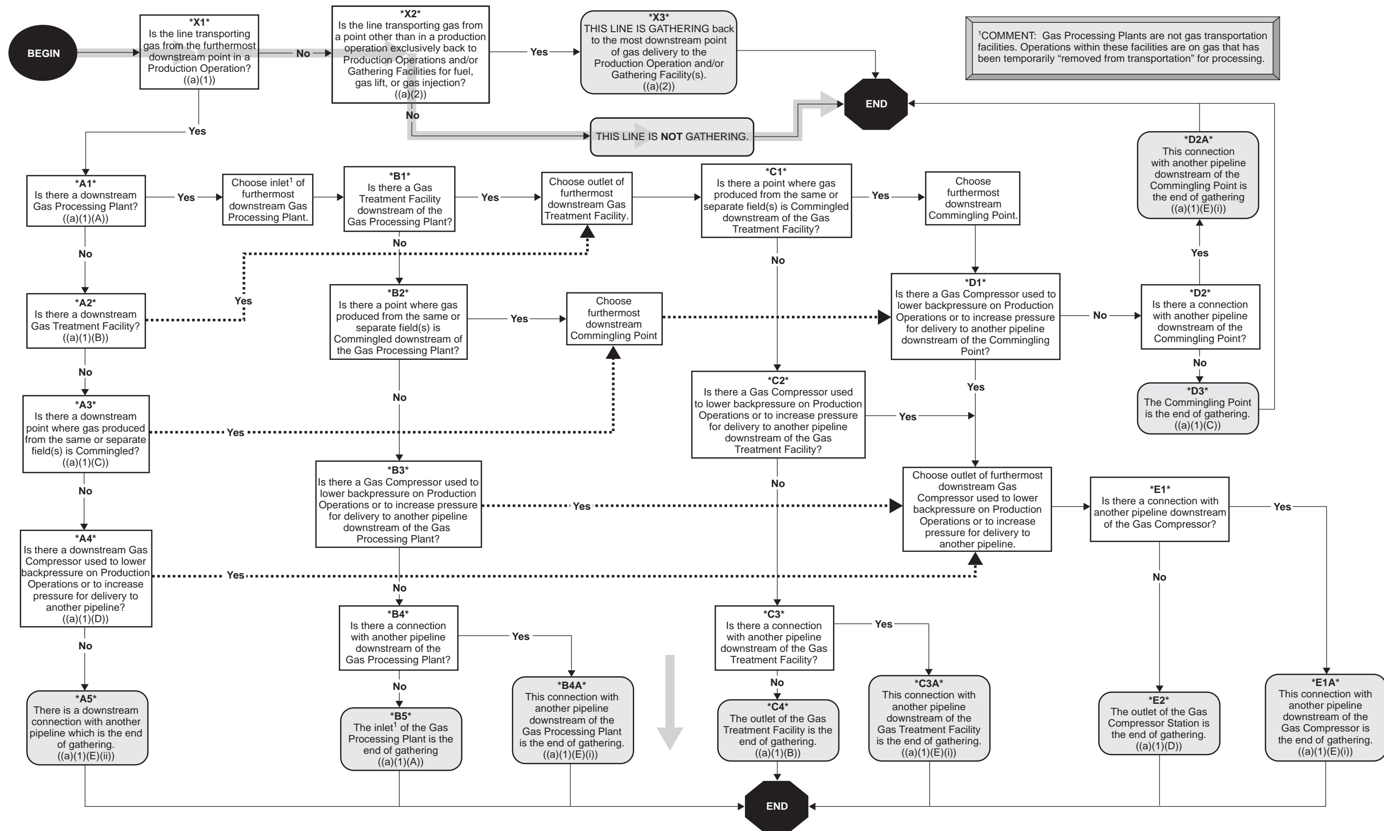
Figure B-7—Alternative 2 Decision Tree for Figure B-1 (Scenario C)
