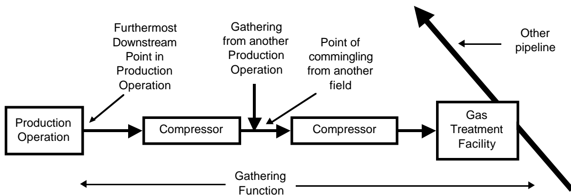
Figure 2-5—Gathering Extends to the Futhermost Downstream Endpoint
