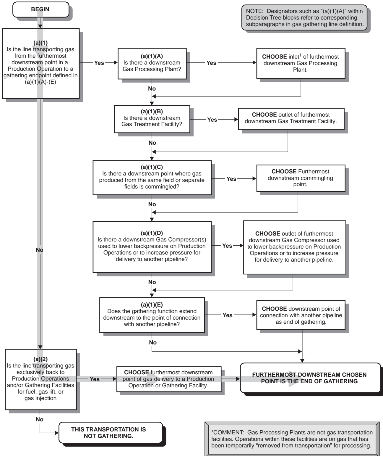
Figure B-18—Alternative 1 Decision Tree for Figure B-17 (Gas Return Lines)
