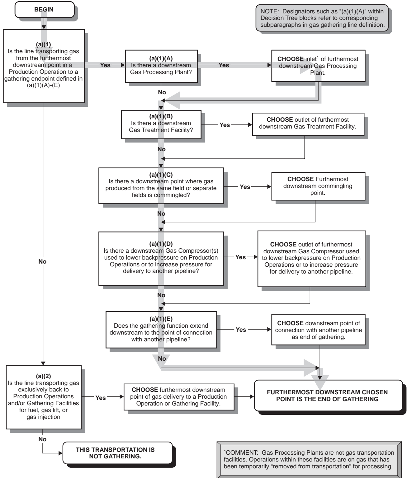
Figure B-20—Alternative 1 Decision Tree for Figure B-17 (Production Gathering)
