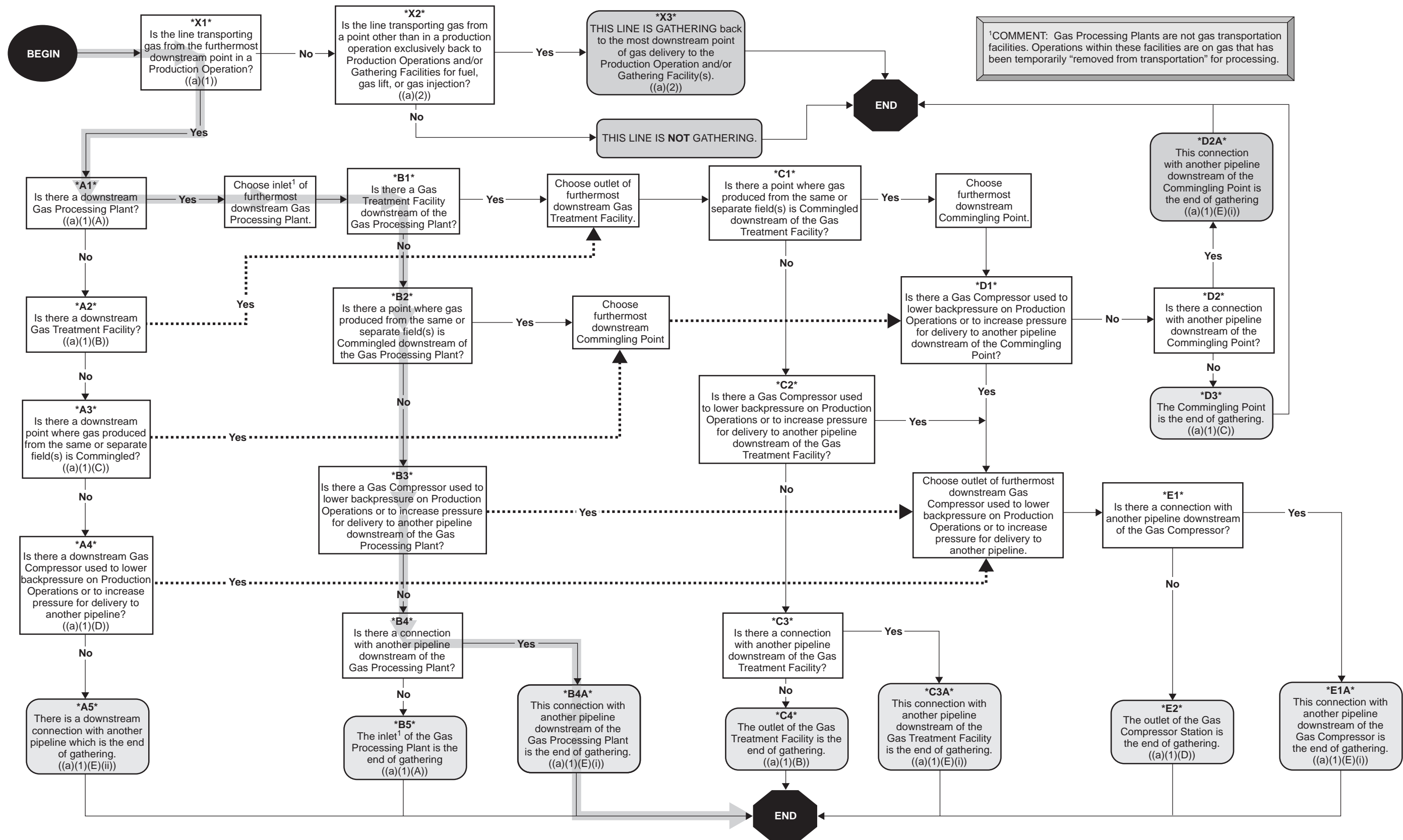
Figure B-3—Alternative 2 Decision Tree for Figure B-1 (Scenario A)
