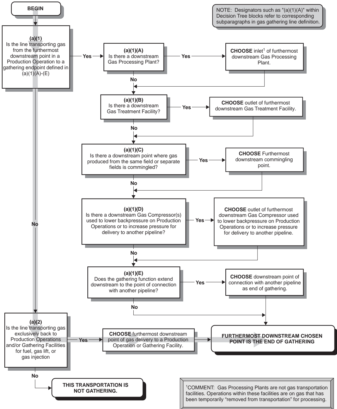
Figure B-9—Alternative 1 Decision Tree for Figure B-8
