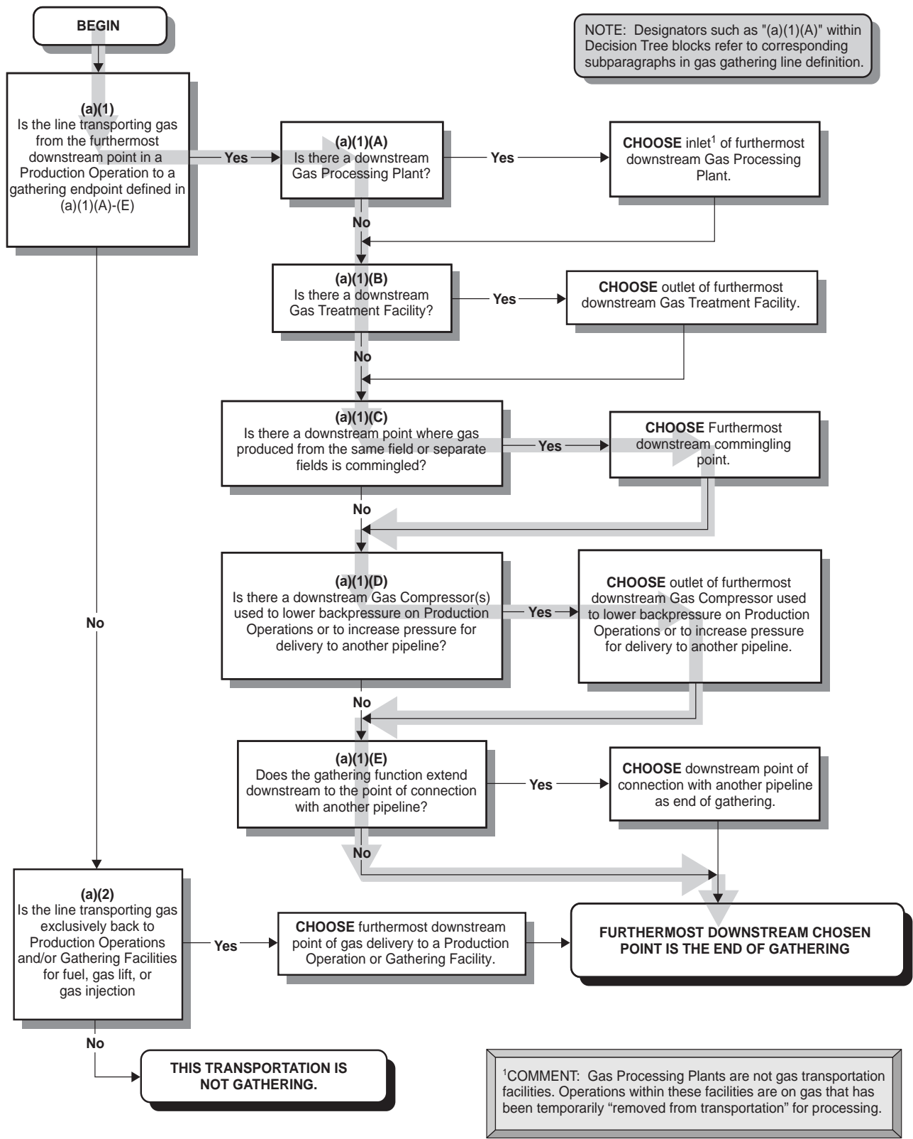
Figure B-15—Alternative 1 Decision Tree for Figure B-14
