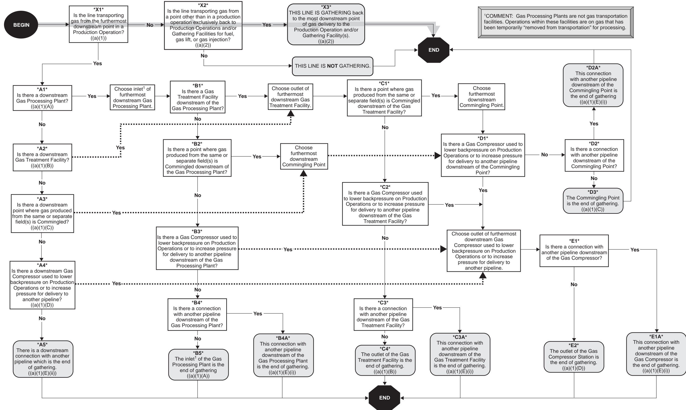
Figure B-19—Alternative 2 Decision Tree for Figure B-17 (Gas Return Lines)
