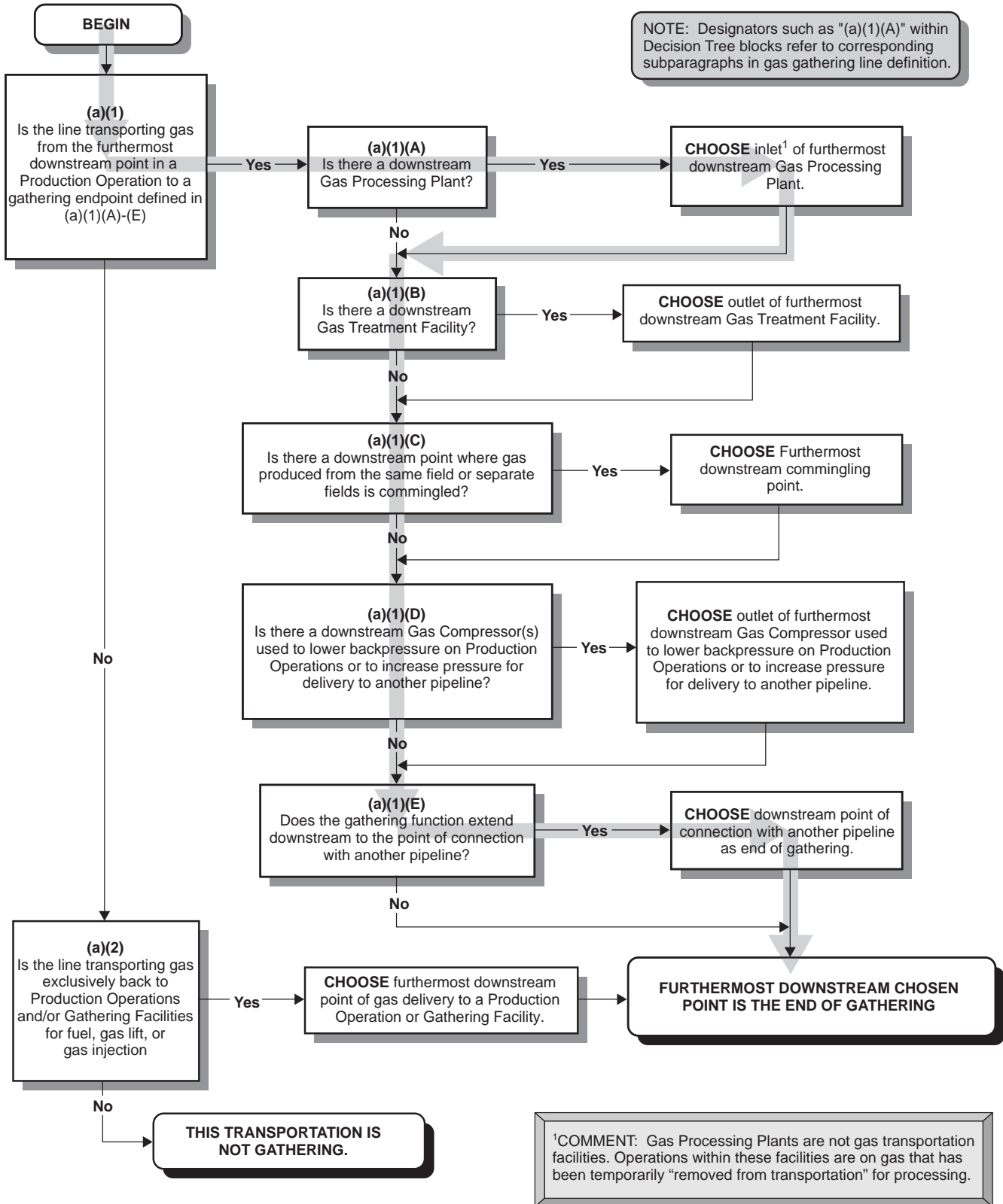
Figure B-2—Alternative1 Decision Tree for Figure B-1 (Scenario A)
