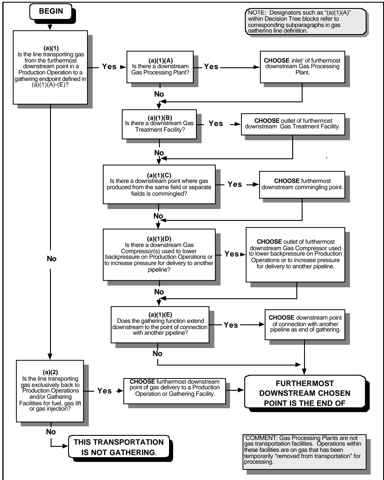
Figure A-1—Onshore Gas Gathering Decision Tree—Alternative 1
