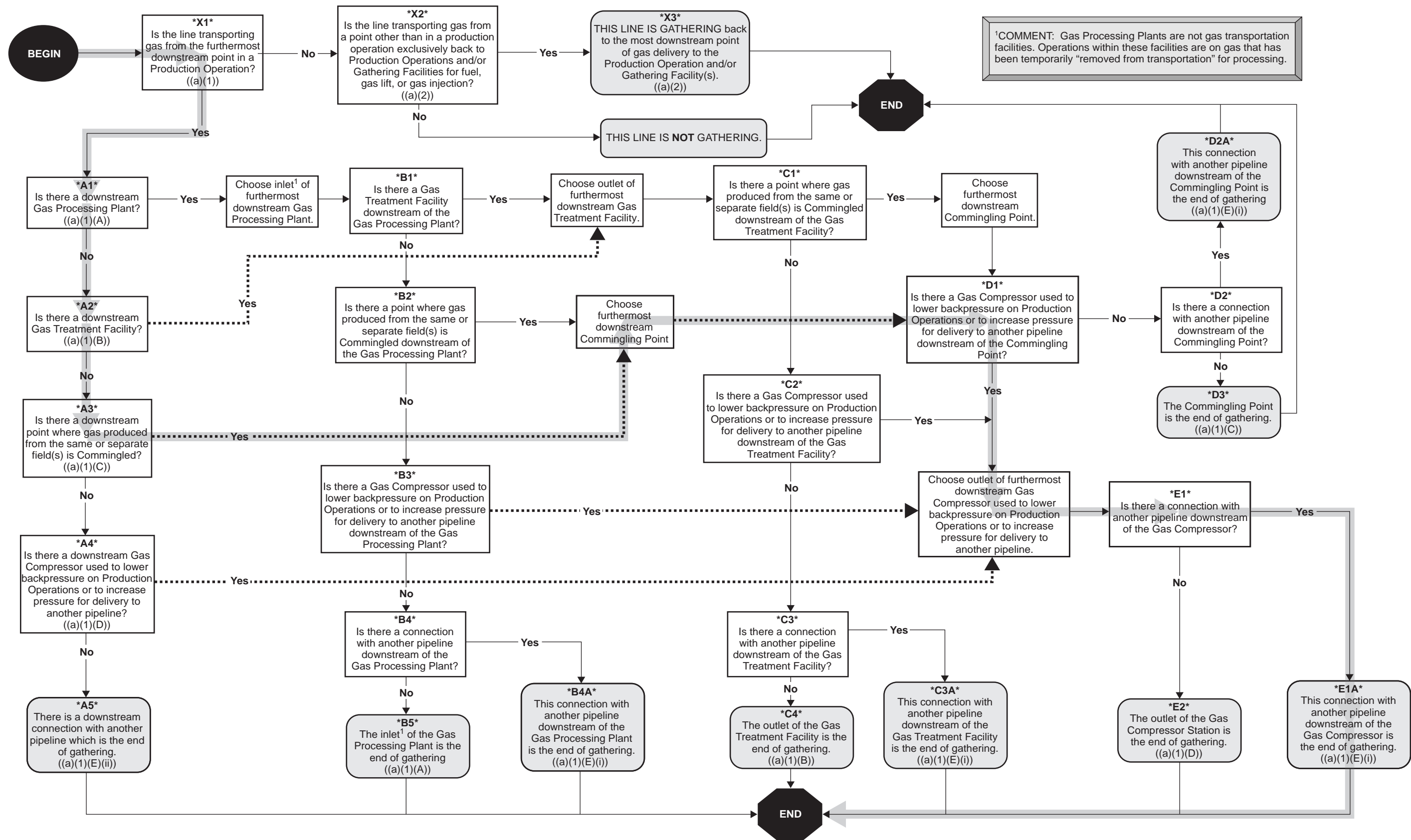
Figure B-13—Alternative 2 Decision Tree for Figure B-11
