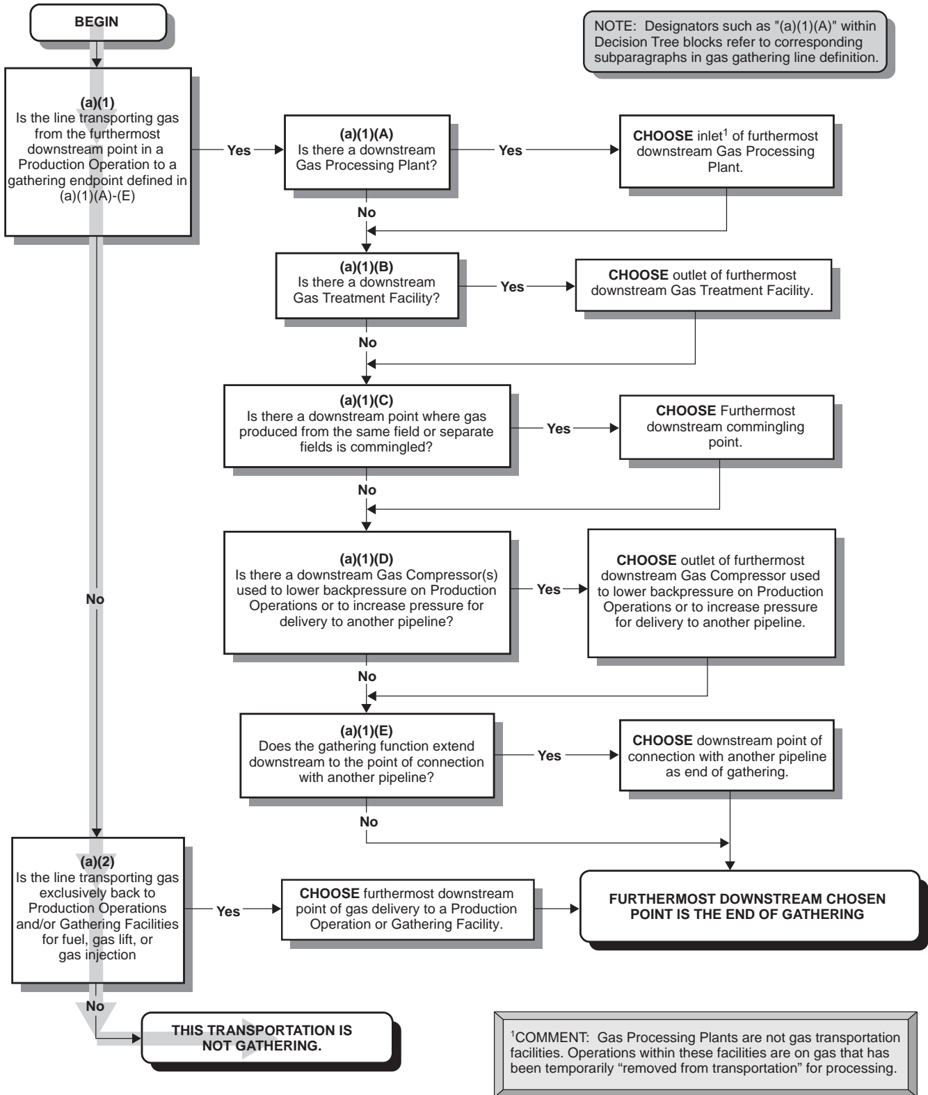
Figure B-6—Alternative 1 Decision Tree for Figure B-1 (Scenario C)
